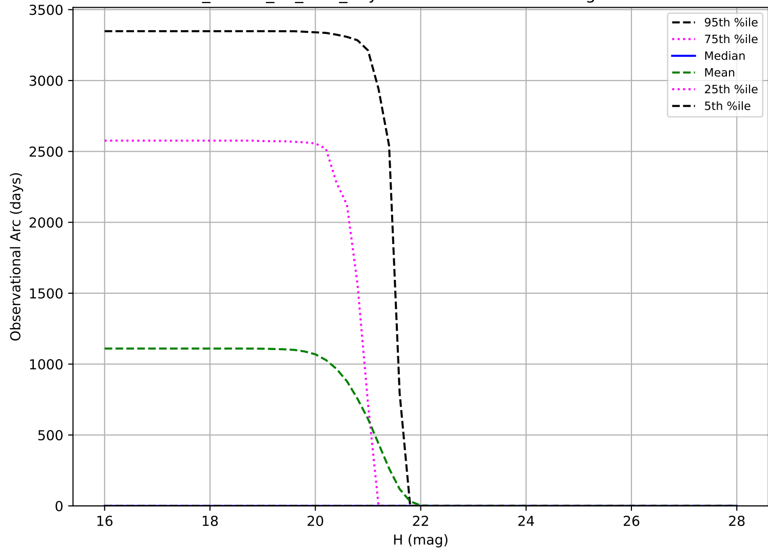
ddf_loaded_fl1_v3.4_10yrs: Observational Arc Length Vatra
