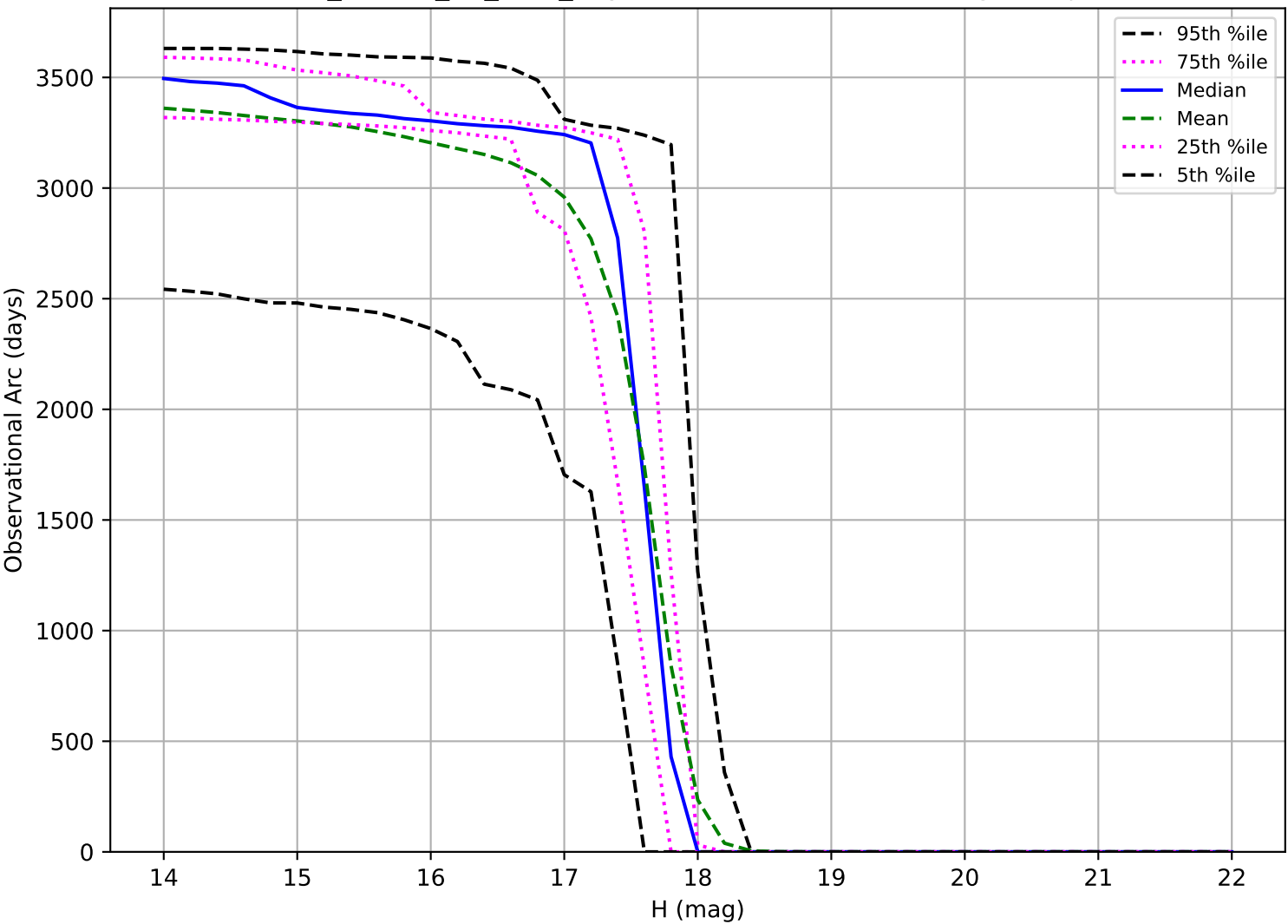
ddf_loaded_fl1_v3.4_10yrs: Observational Arc Length Trojan
