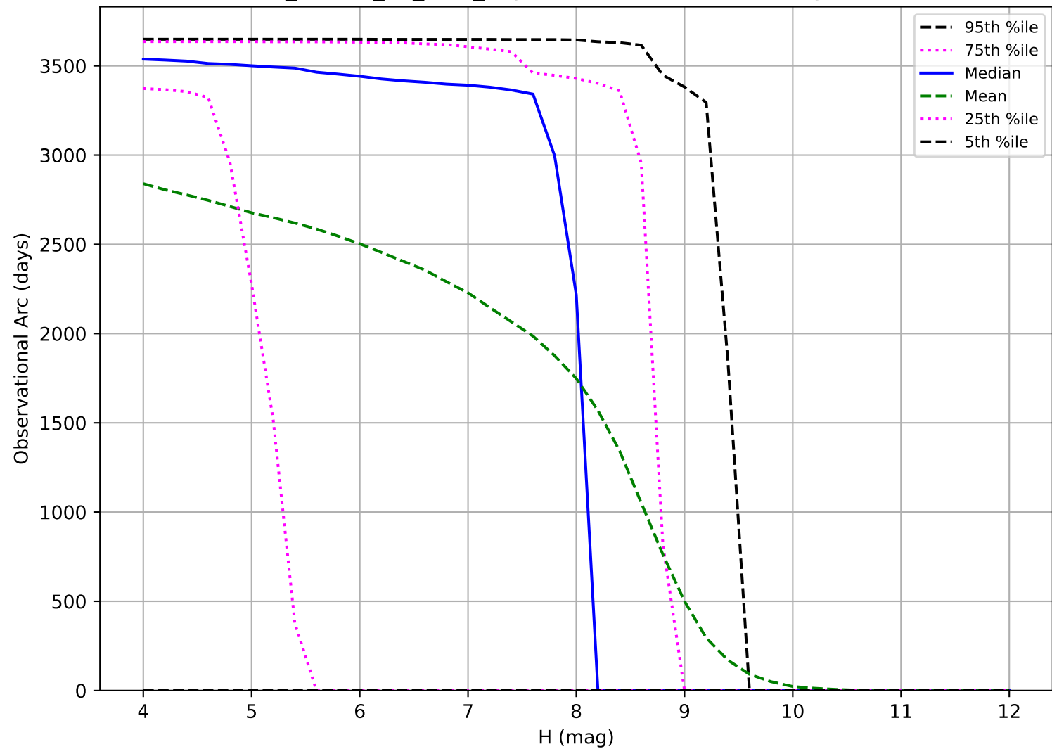
ddf_loaded_fl1_v3.4_10yrs: Observational Arc Length TNO
