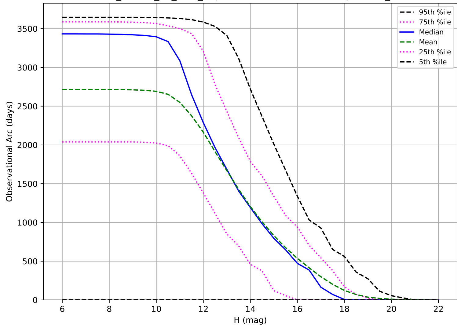
ddf_loaded_fl1_v3.4_10yrs: Observational Arc Length OCC_r5
