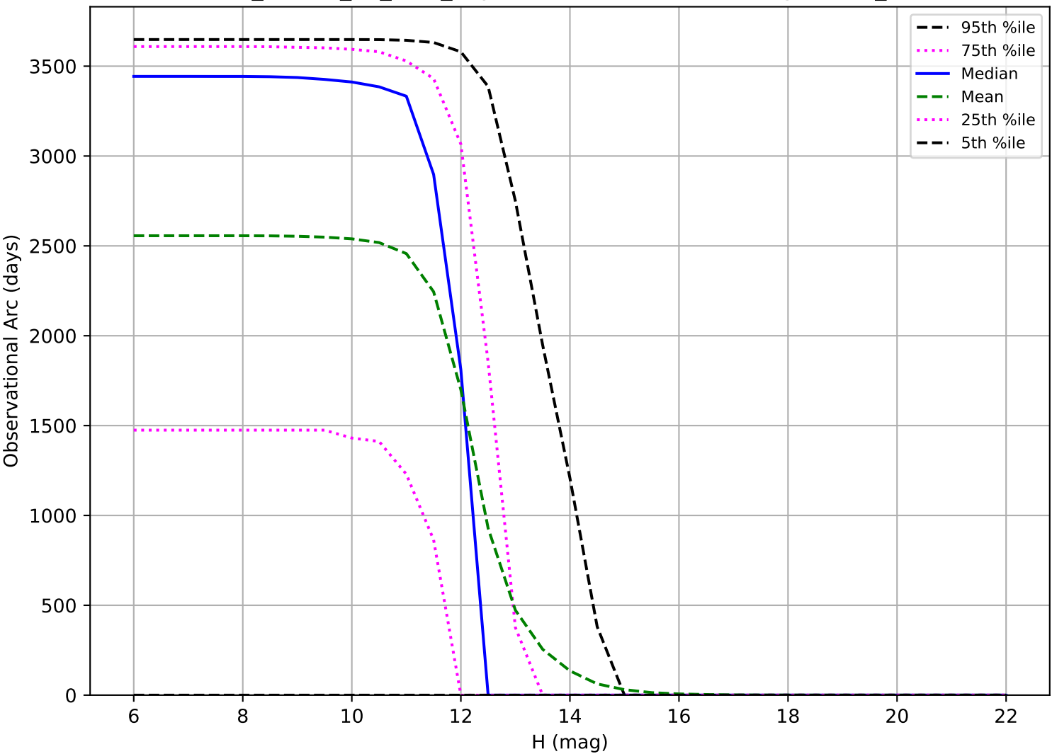
ddf_loaded_fl1_v3.4_10yrs: Observational Arc Length OCC_r20
