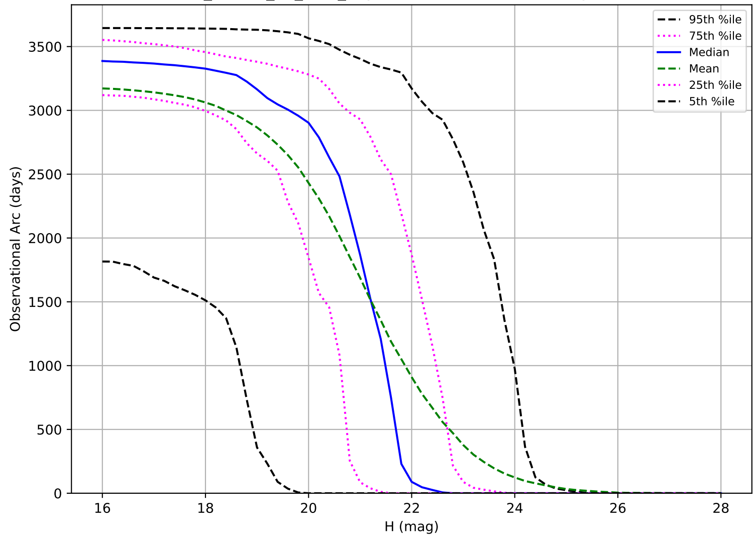
ddf_loaded_fl1_v3.4_10yrs: Observational Arc Length NEO
