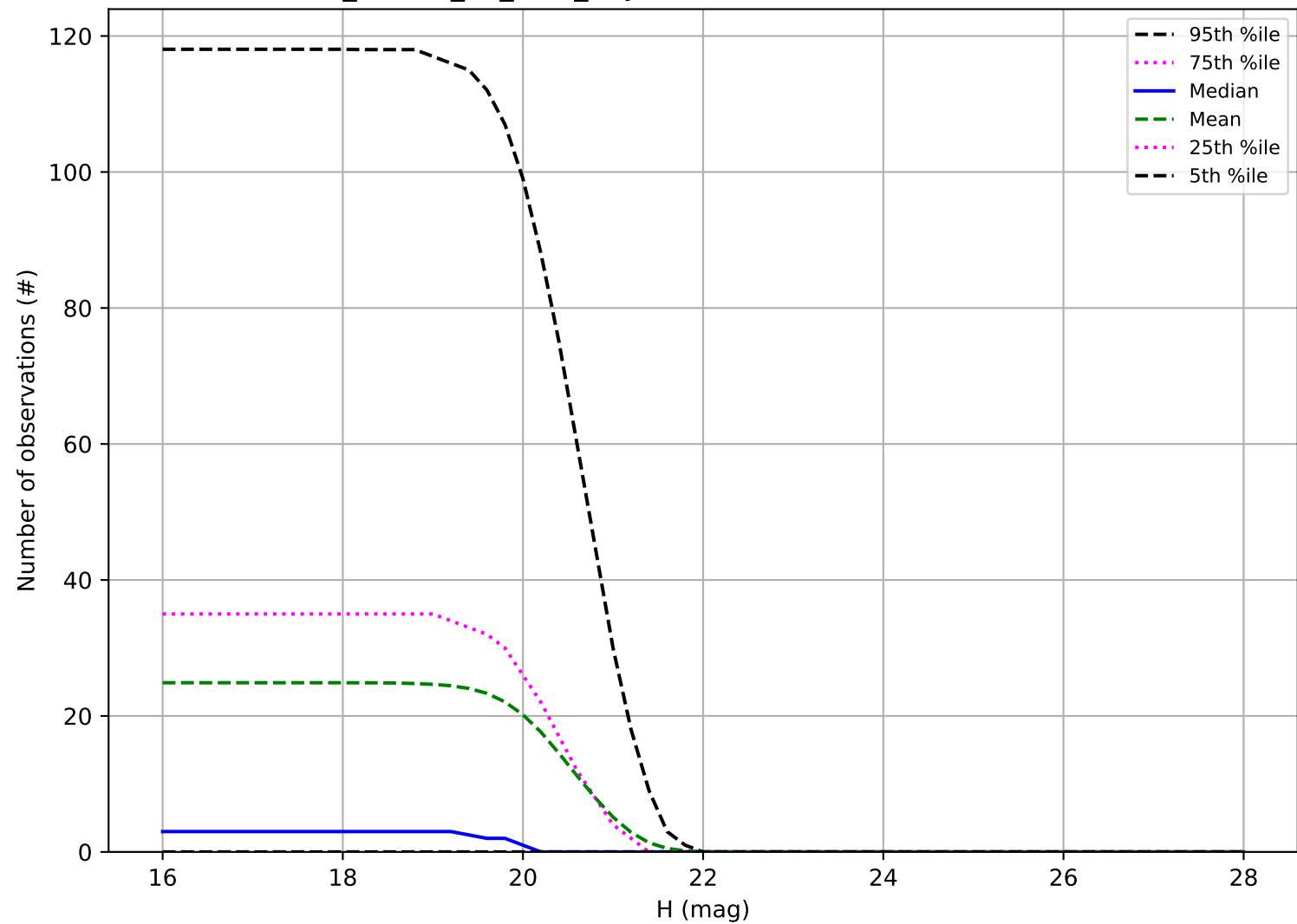
ddf_loaded_fl1_v3.4_10yrs: Number of observations Vatira
