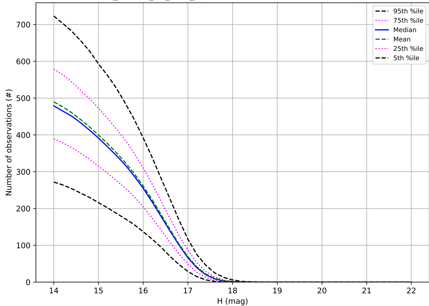
ddf_loaded_fl1_v3.4_10yrs: Number of observations Trojan
