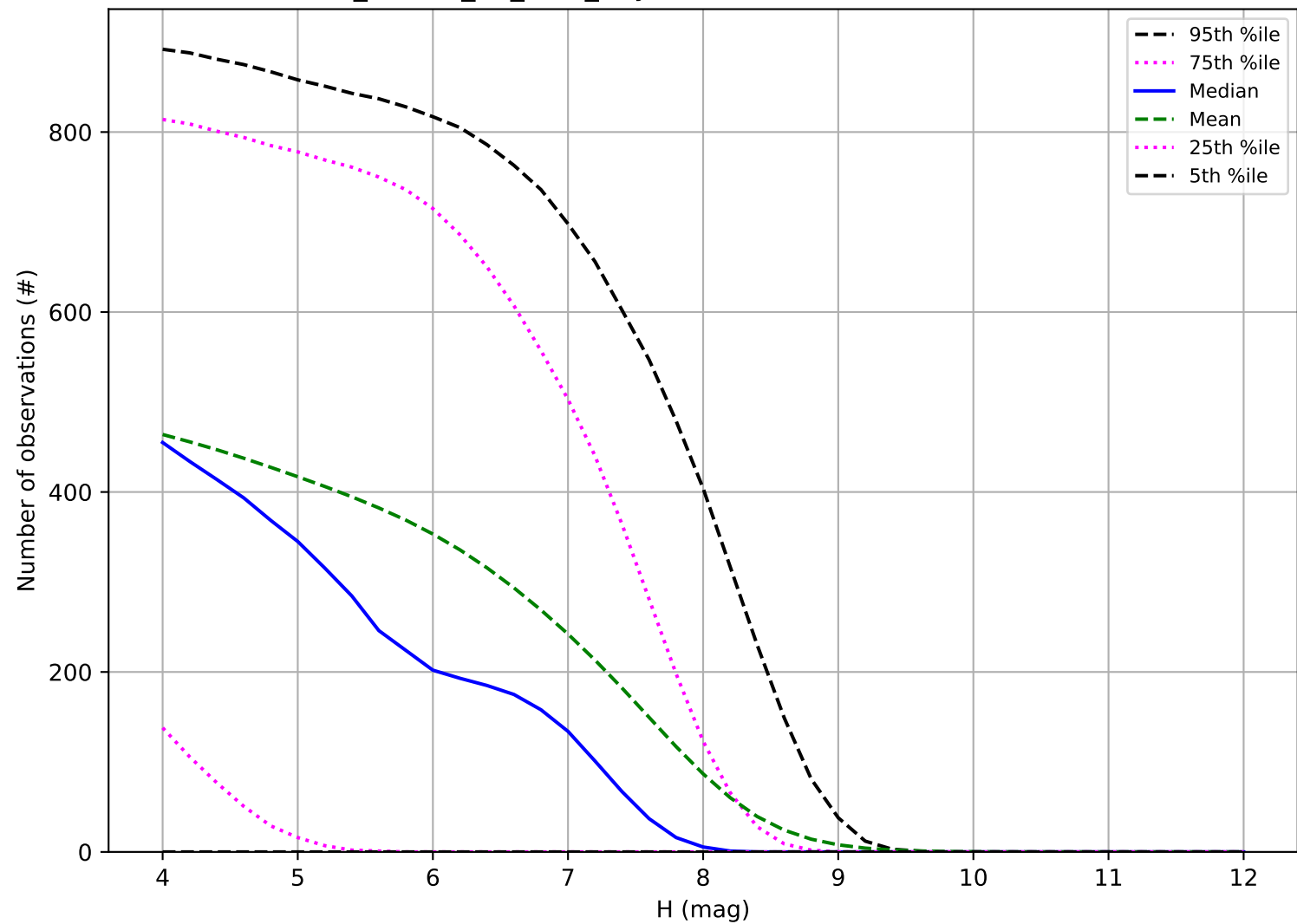
ddf_loaded_fl1_v3.4_10yrs: Number of observations TNO
