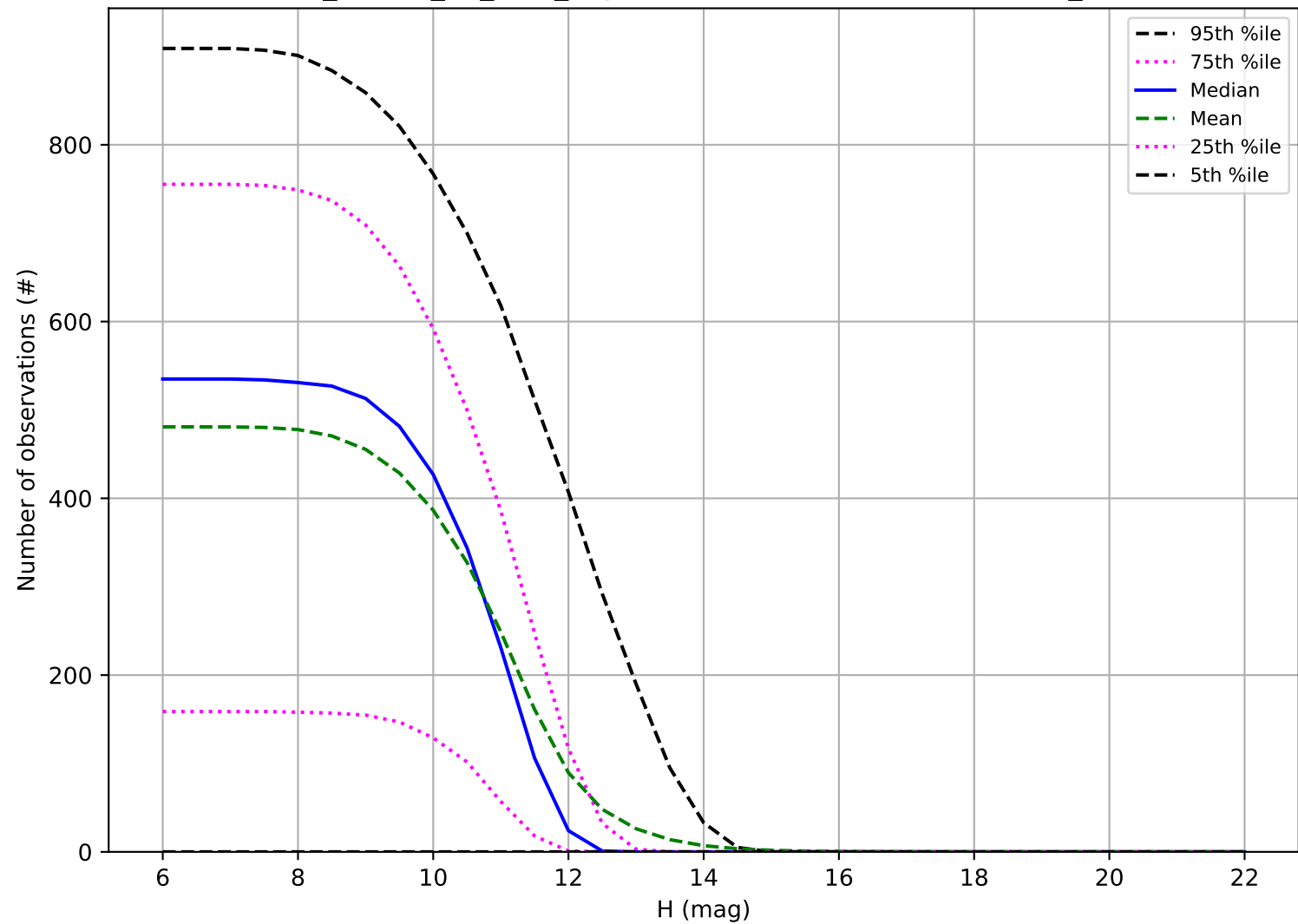
ddf_loaded_fl1_v3.4_10yrs: Number of observations OCC_r20
