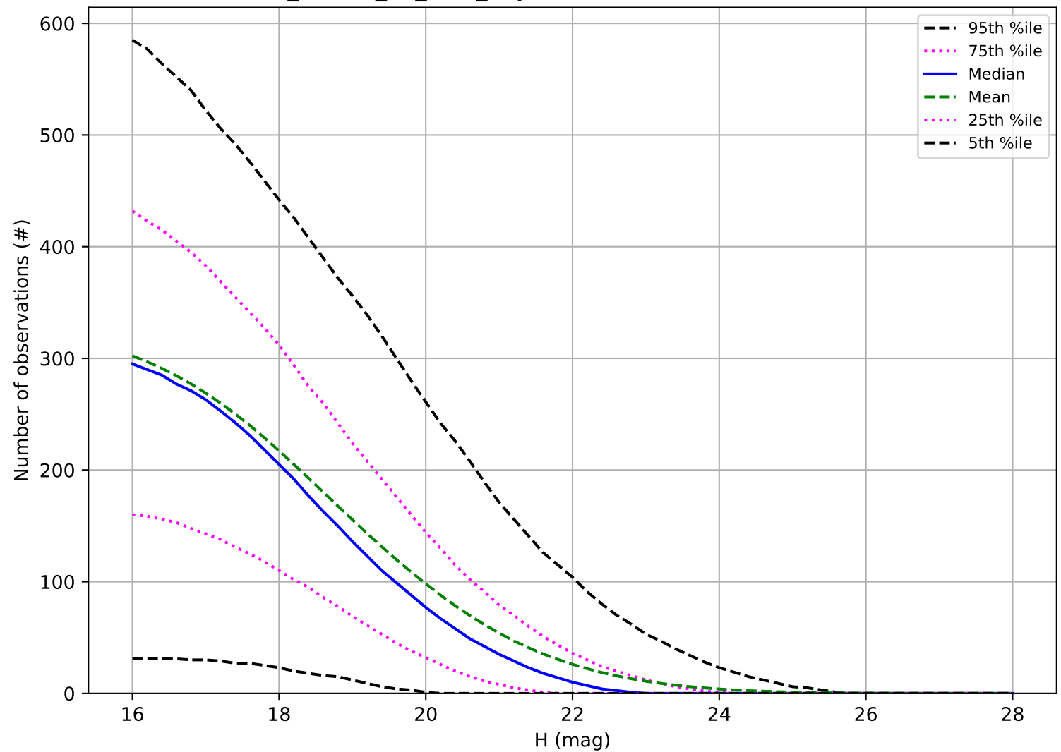
ddf_loaded_fl1_v3.4_10yrs: Number of observations NEO
