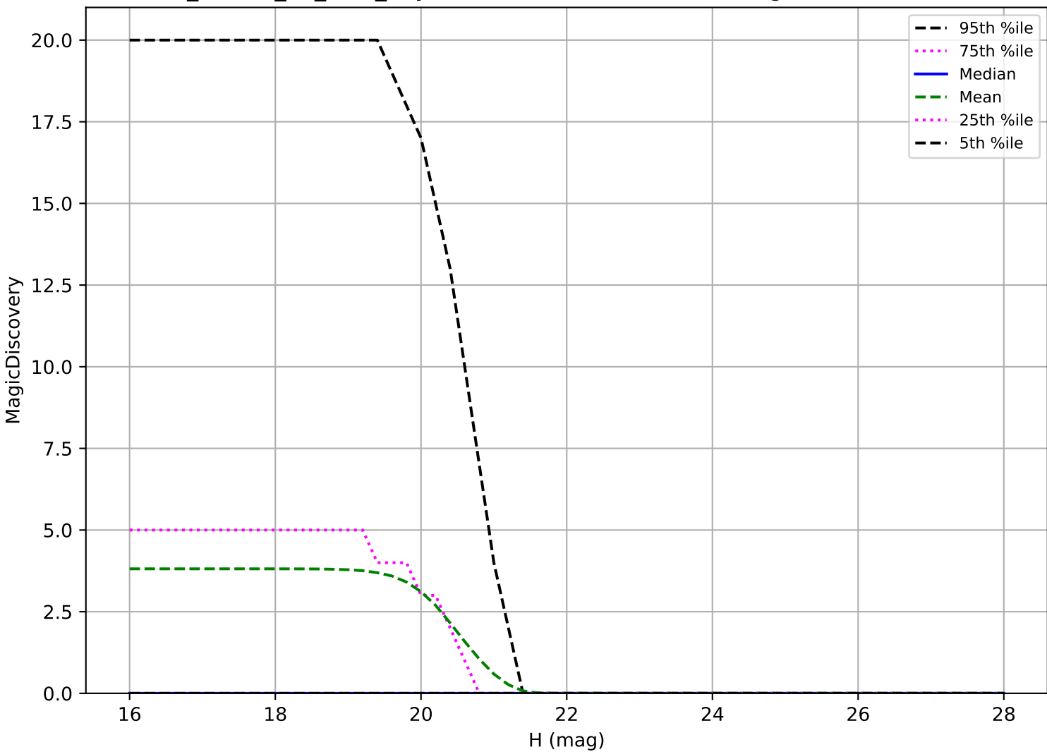
ddf_loaded_fl1_v3.4_10yrs: Vatira 6 detections in 60 nights detection loss
