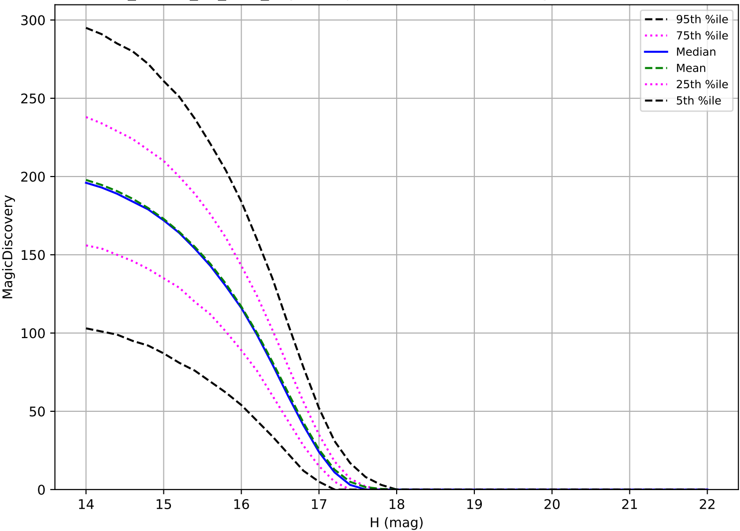
ddf_loaded_fl1_v3.4_10yrs: Trojan 6 detections in 60 nights detection loss
