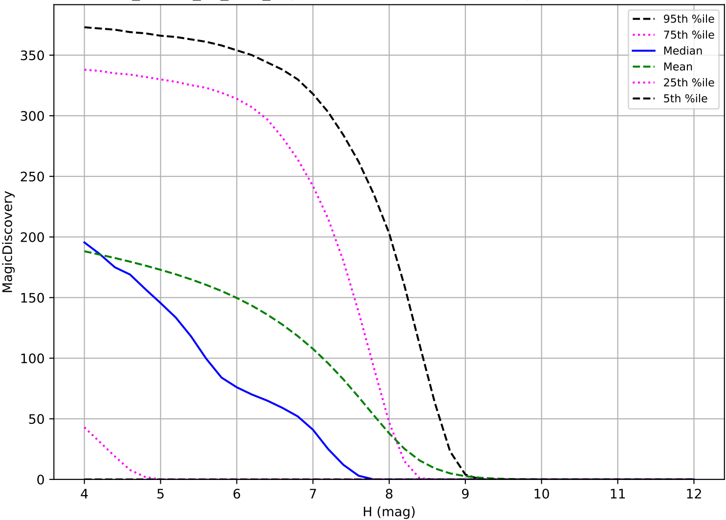
ddf_loaded_fl1_v3.4_10yrs: TNO 6 detections in 60 nights detection loss
