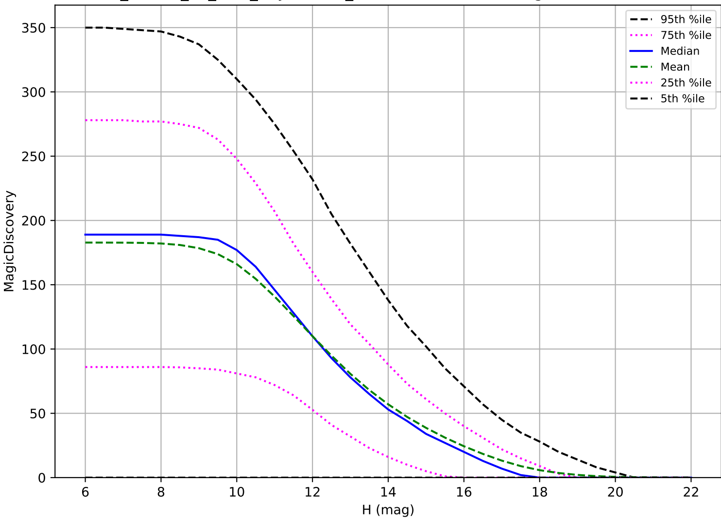
ddf_loaded_fl1_v3.4_10yrs: OCC_r5 6 detections in 60 nights detection loss
