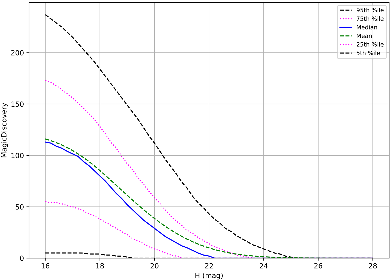
ddf_loaded_fl1_v3.4_10yrs: NEO 6 detections in 60 nights detection loss
