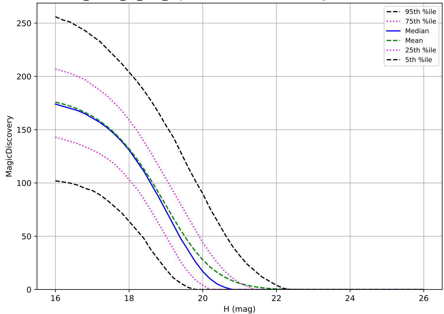
ddf_loaded_fl1_v3.4_10yrs: MBA 6 detections in 60 nights detection loss
