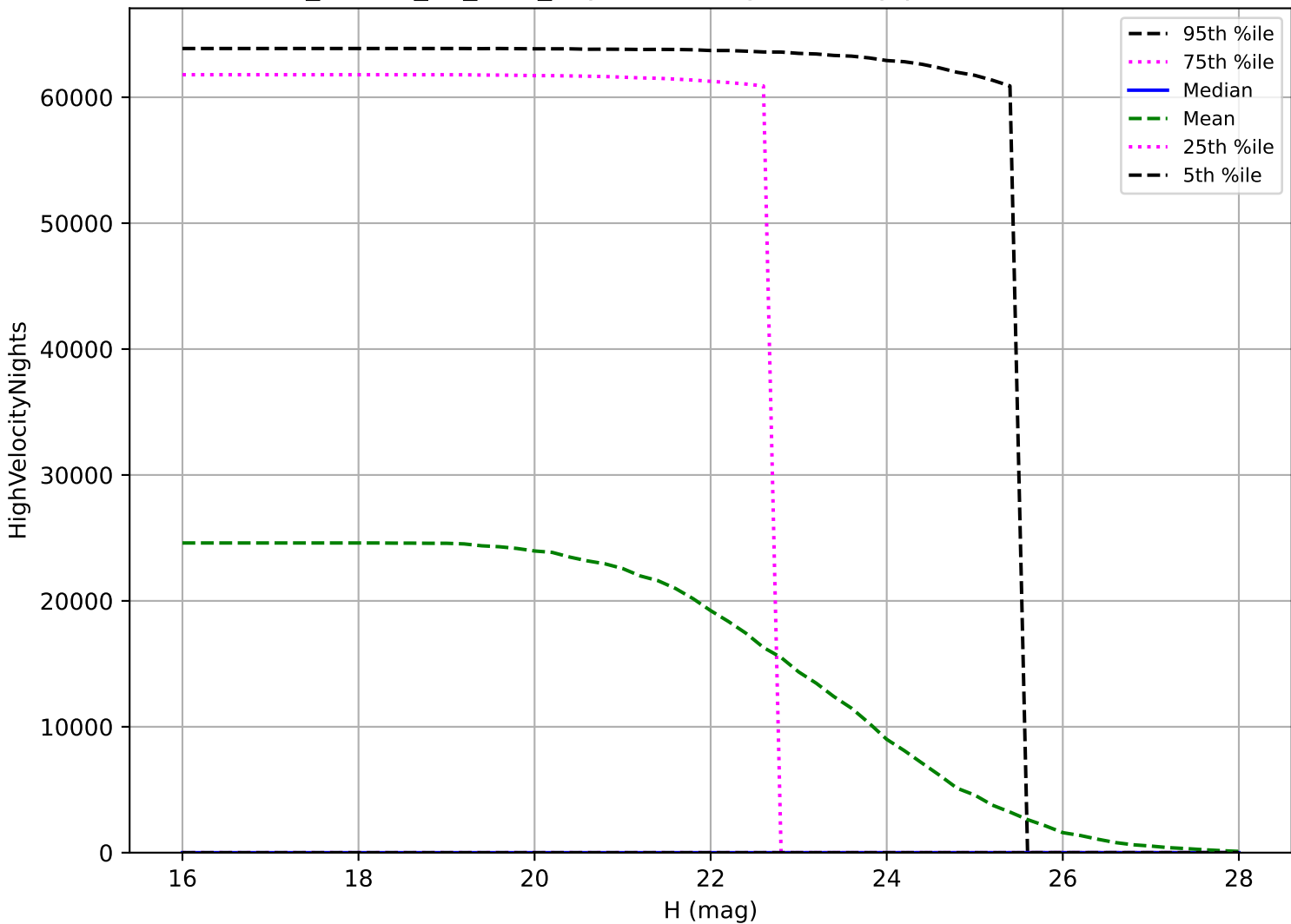
ddf_loaded_fl1_v3.4_10yrs: PHA High velocity pair detection loss
