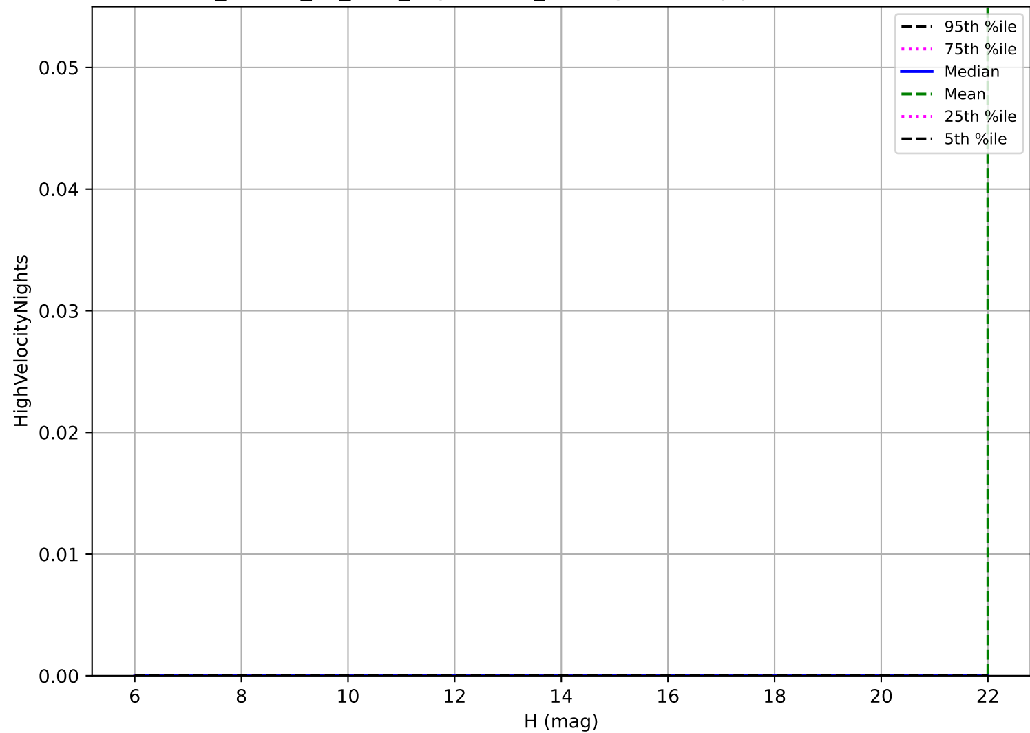
ddf_loaded_fl1_v3.4_10yrs: OCC_r20 High velocity pair detection loss
