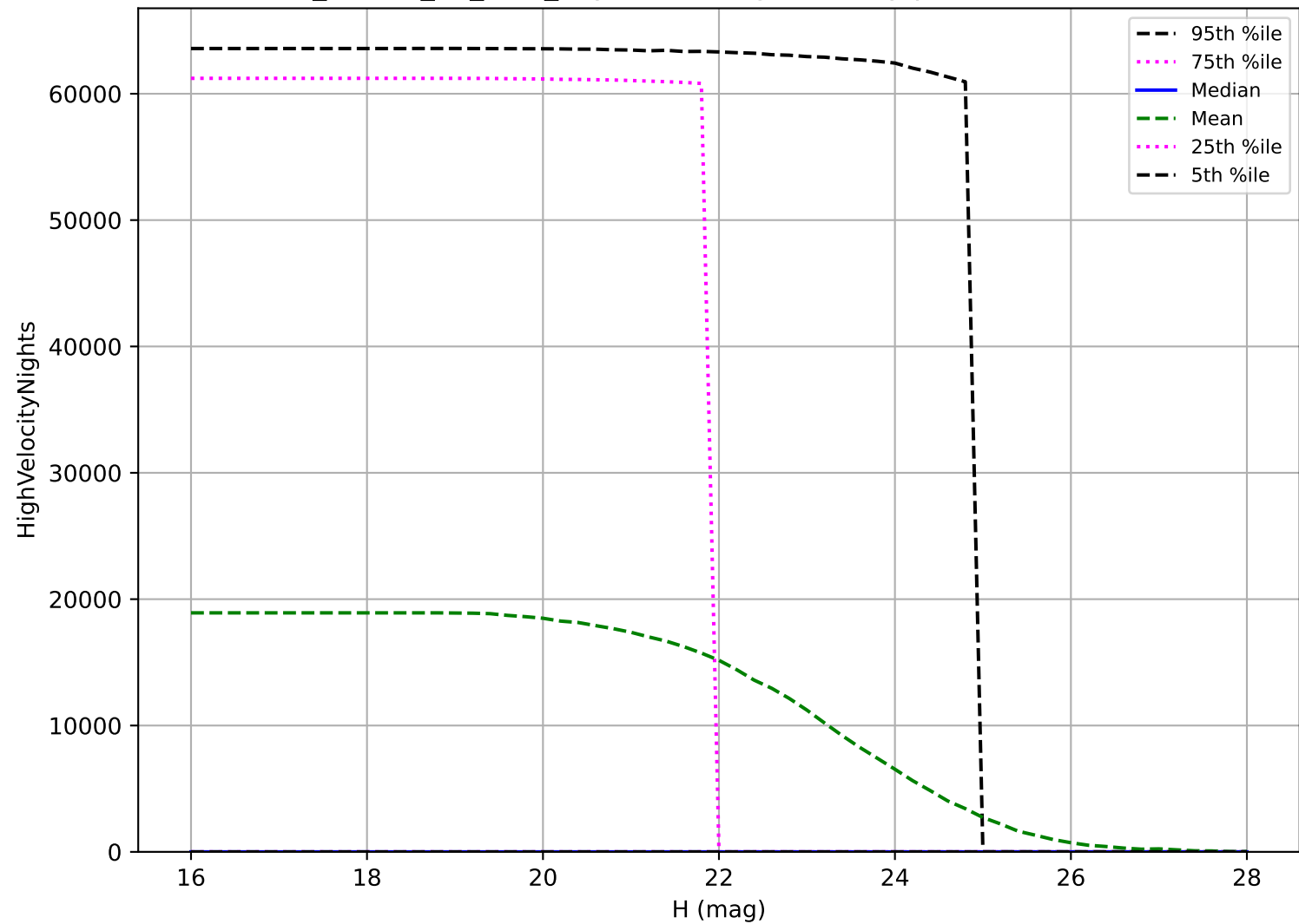
ddf_loaded_fl1_v3.4_10yrs: NEO High velocity pair detection loss
