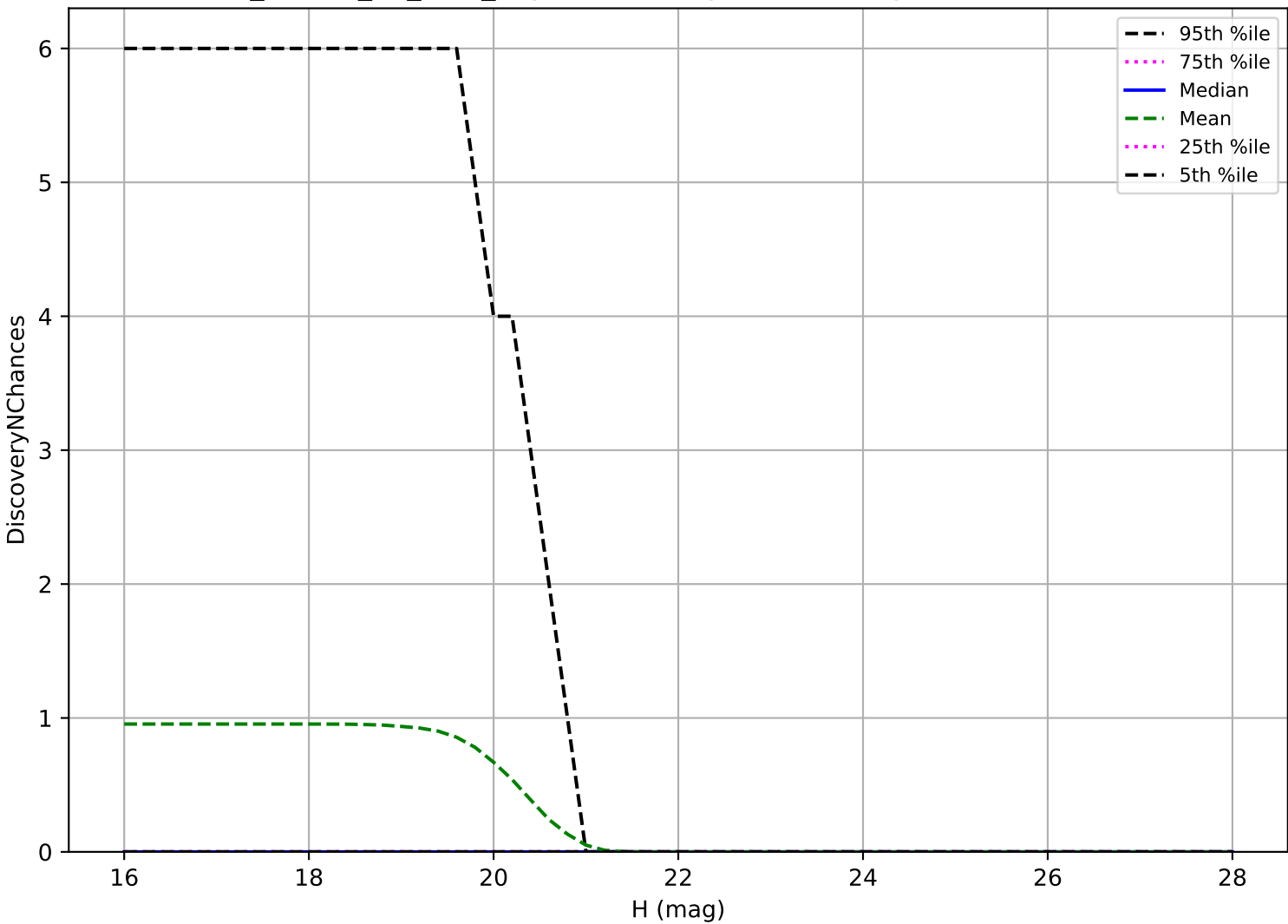
ddf_loaded_fl1_v3.4_10yrs: Vatira 3 pairs in 15 nights detection loss
