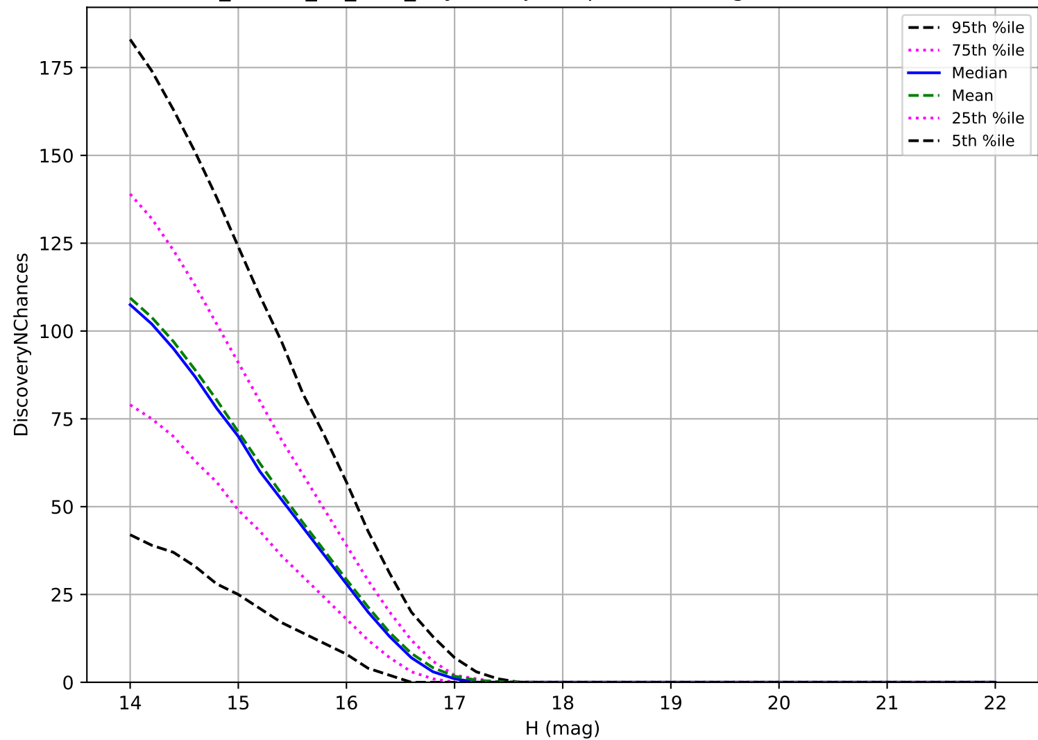
ddf_loaded_fl1_v3.4_10yrs: Trojan 3 pairs in 15 nights detection loss
