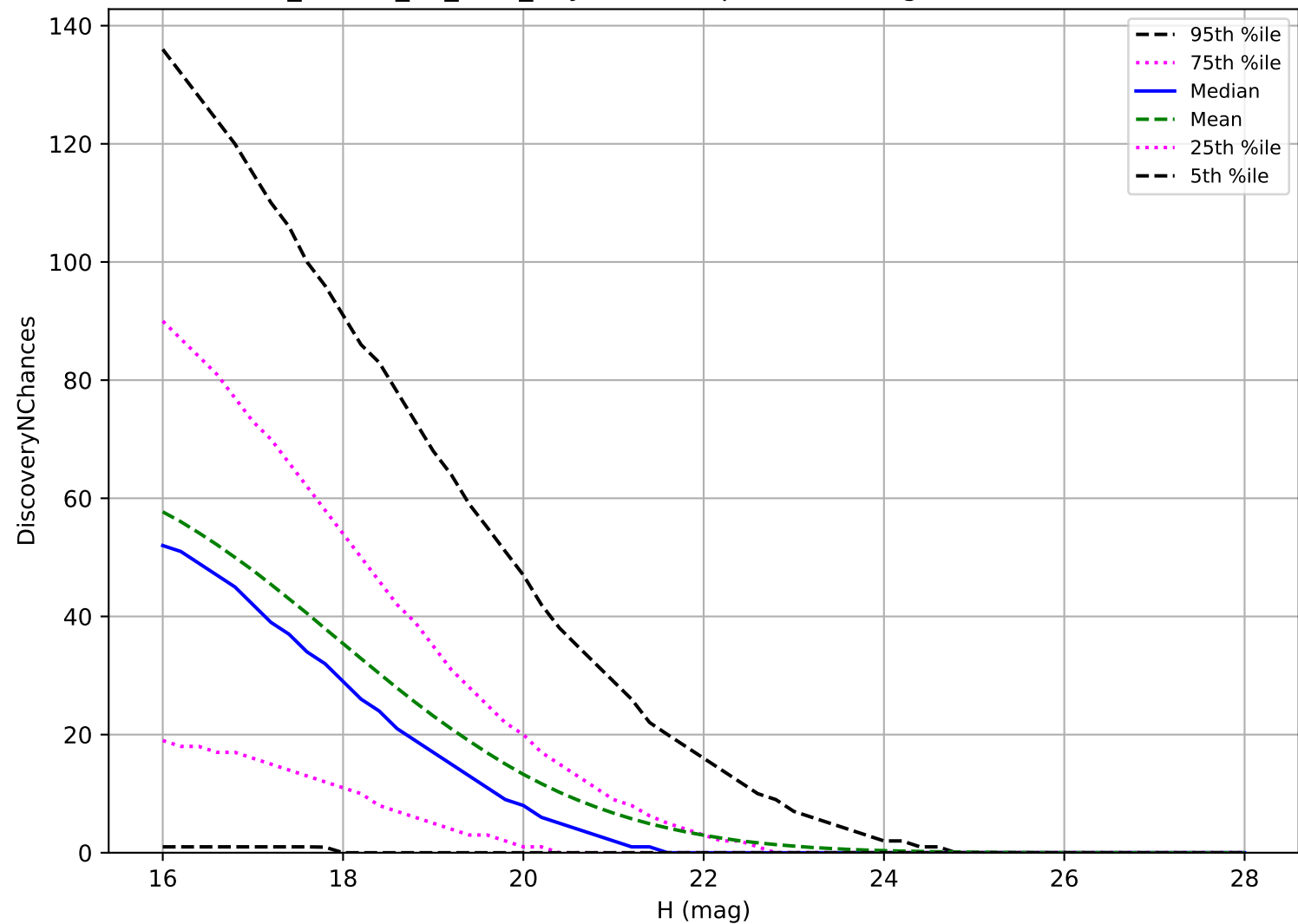
ddf_loaded_fl1_v3.4_10yrs: PHA 3 pairs in 15 nights detection loss
