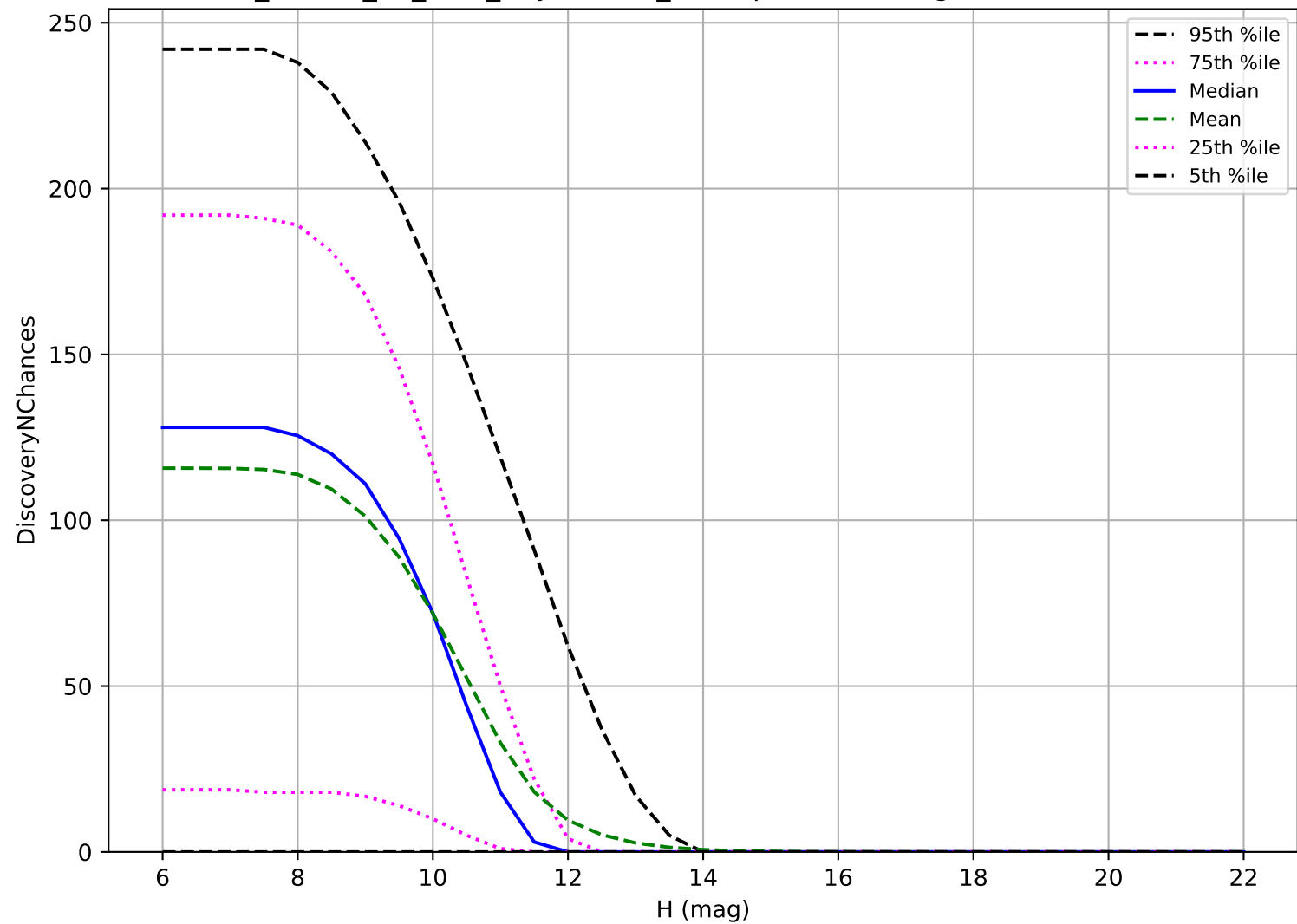
ddf_loaded_fl1_v3.4_10yrs: OCC_r20 3 pairs in 15 nights detection loss
