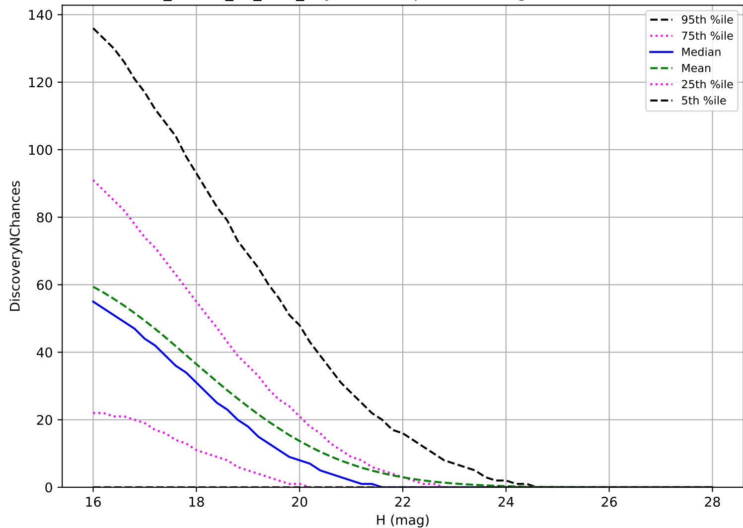
ddf_loaded_fl1_v3.4_10yrs: NEO 3 pairs in 15 nights detection loss
