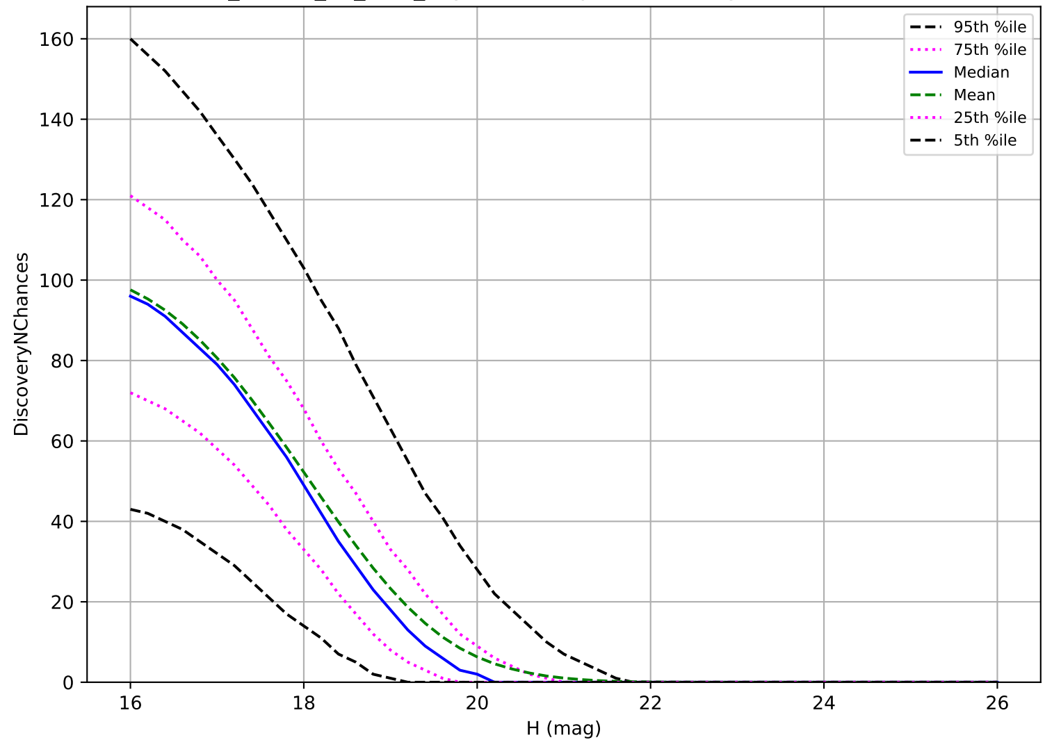
ddf_loaded_fl1_v3.4_10yrs: MBA 3 pairs in 15 nights detection loss
