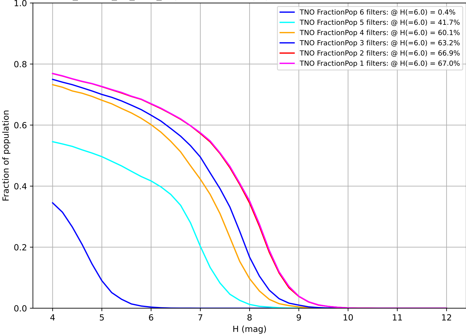
ddf_loaded_fl1_v3.4_10yrs: Fraction of population with colors in X filters TNO
