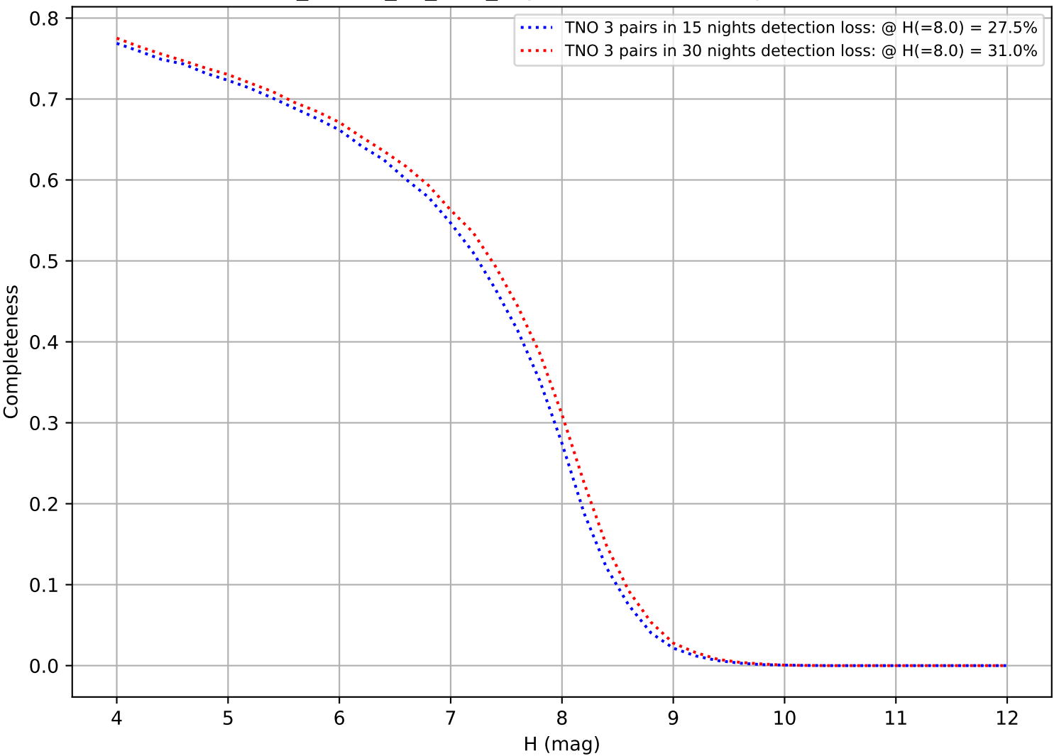
ddf_loaded_fl1_v3.4_10yrs: DifferentialCompleteness
