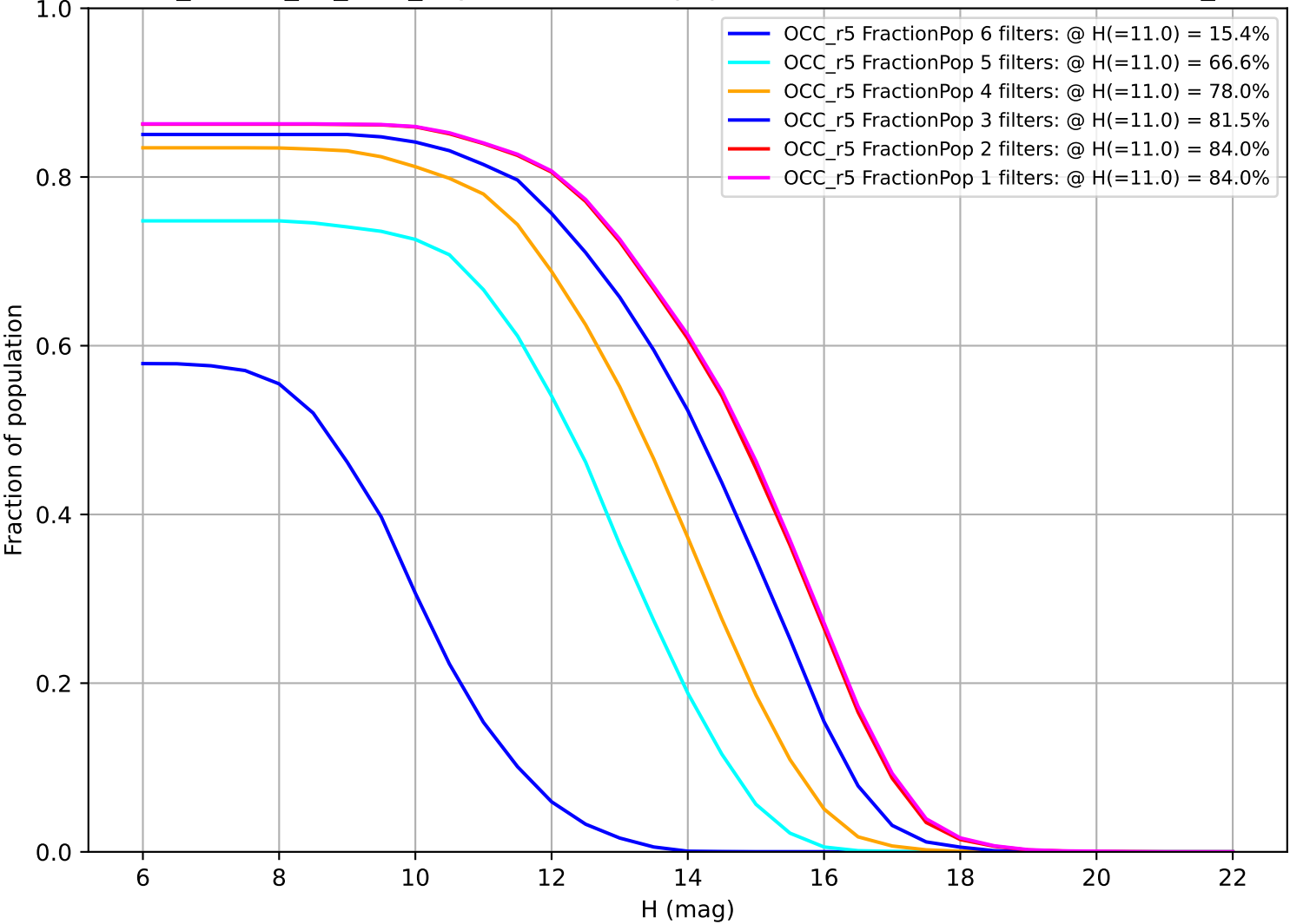
ddf_loaded_fl1_v3.4_10yrs: Fraction of population with colors in X filters OCC_r5
