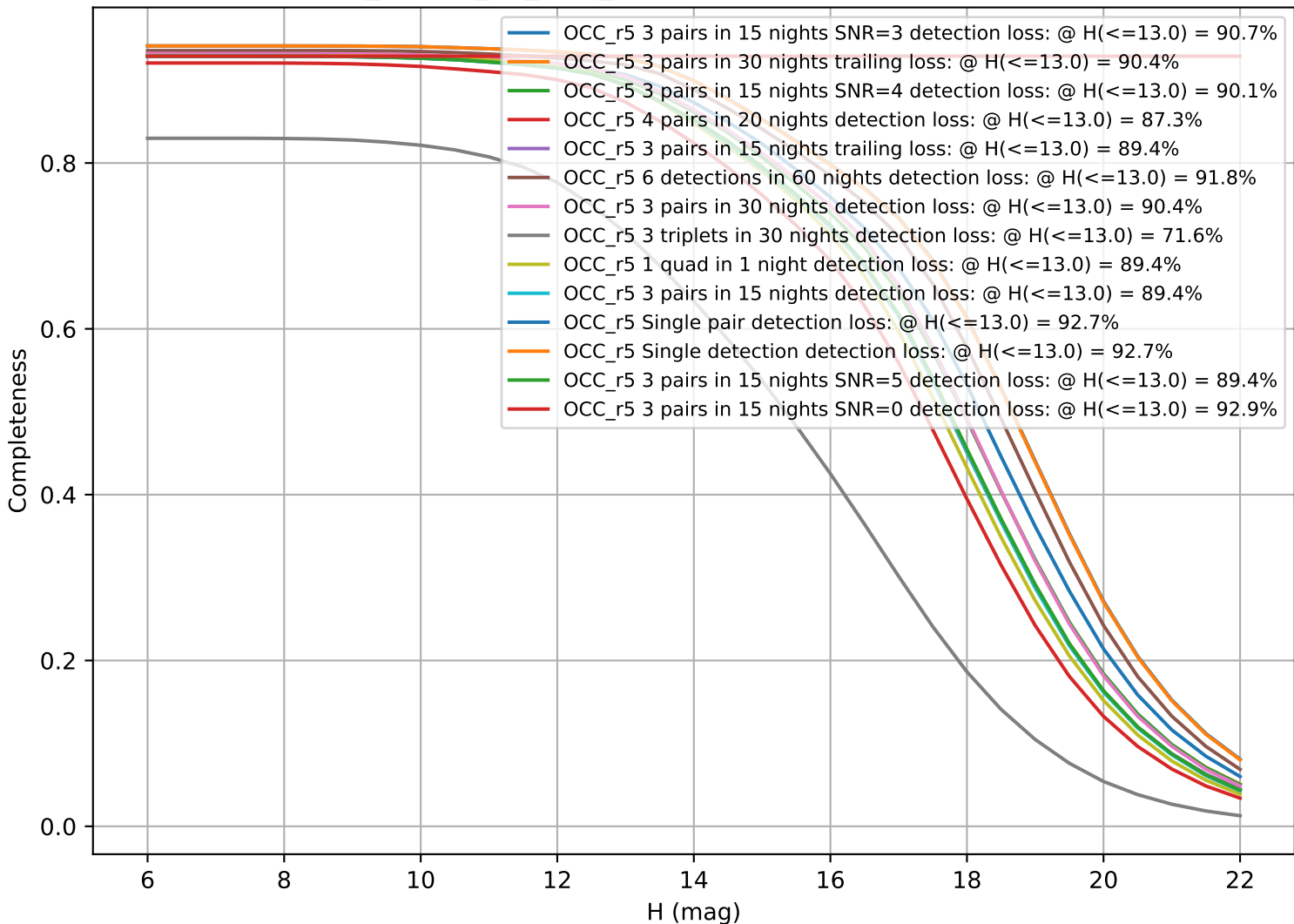
ddf_loaded_fl1_v3.4_10yrs: CumulativeCompleteness
