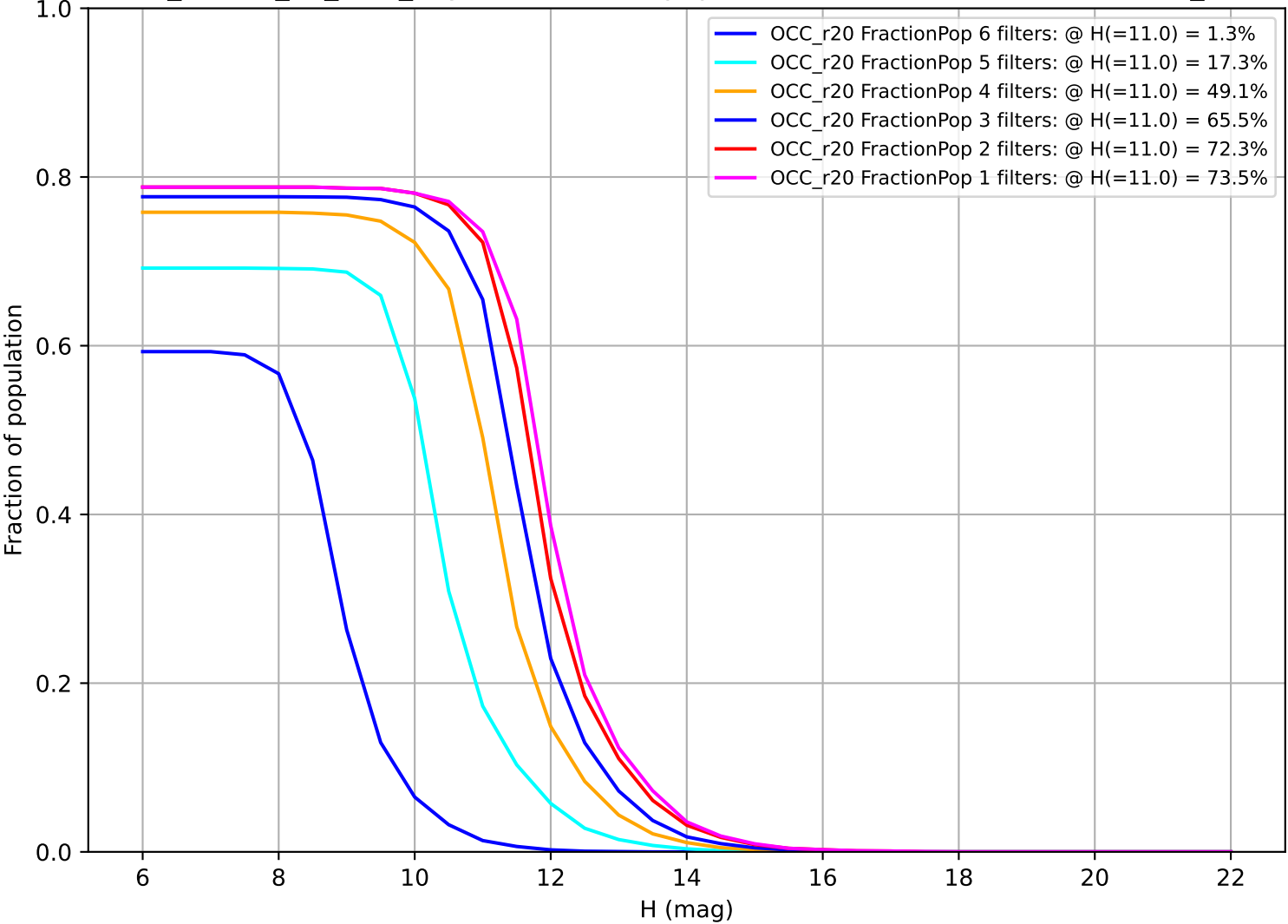
ddf_loaded_fl1_v3.4_10yrs: Fraction of population with colors in X filters OCC_r20
