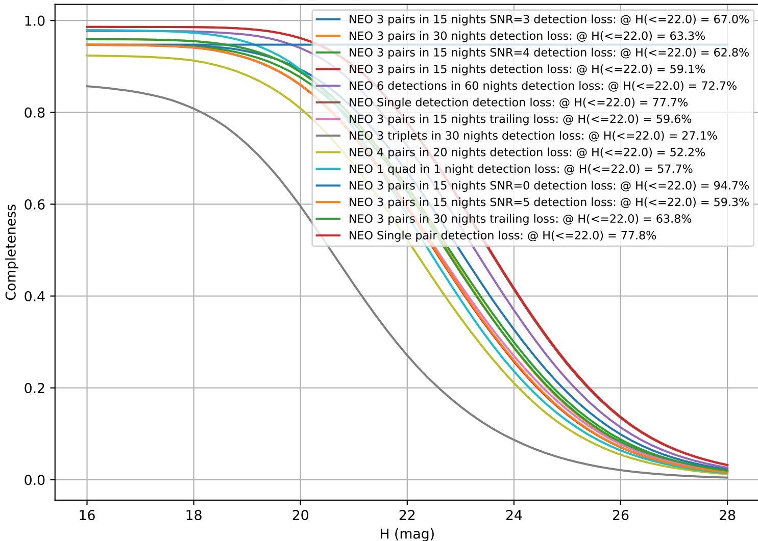
ddf_loaded_fl1_v3.4_10yrs: CumulativeCompleteness
