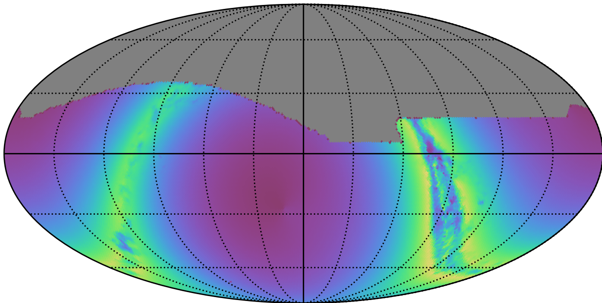
ddf_loaded_fl1_v3.4_10yrs : young_stars
