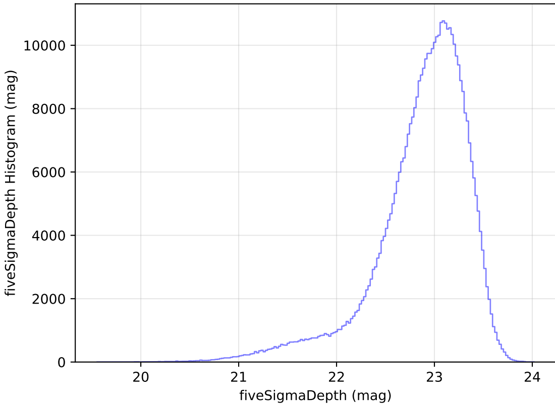
ddf_loaded_fl1_v3.4_10yrs z: fiveSigmaDepth Histogram
