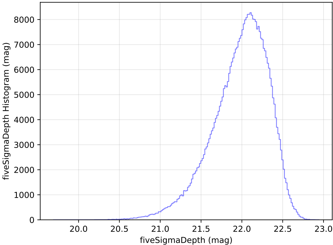
ddf_loaded_fl1_v3.4_10yrs y: fiveSigmaDepth Histogram
