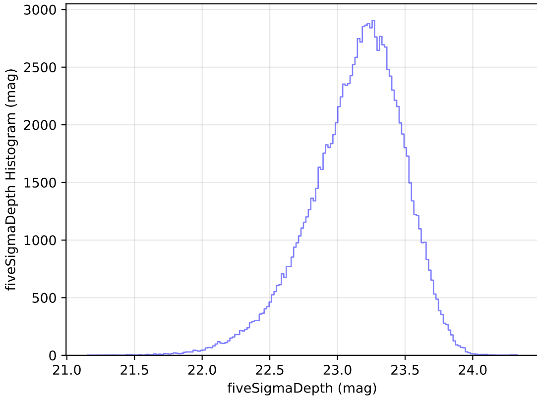
ddf_loaded_fl1_v3.4_10yrs u: fiveSigmaDepth Histogram
