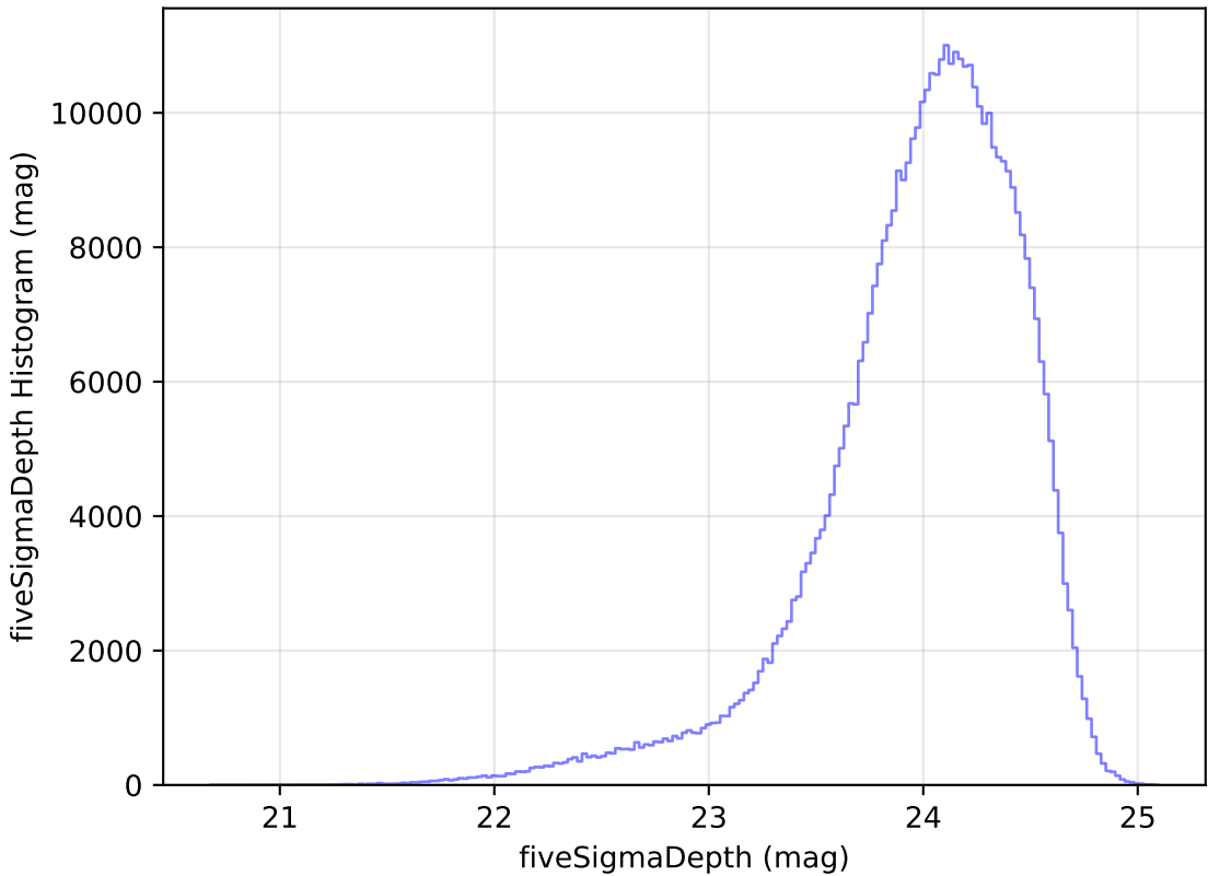
ddf_loaded_fl1_v3.4_10yrs r: fiveSigmaDepth Histogram
