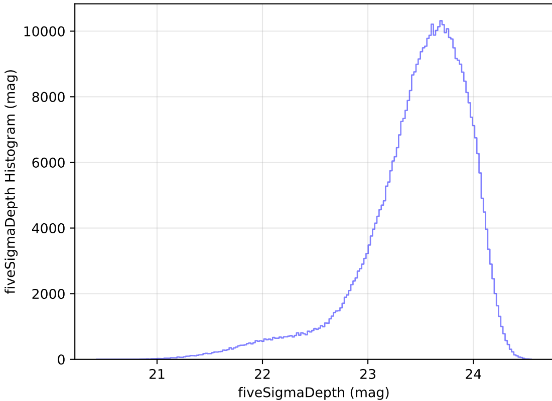
ddf_loaded_fl1_v3.4_10yrs i: fiveSigmaDepth Histogram
