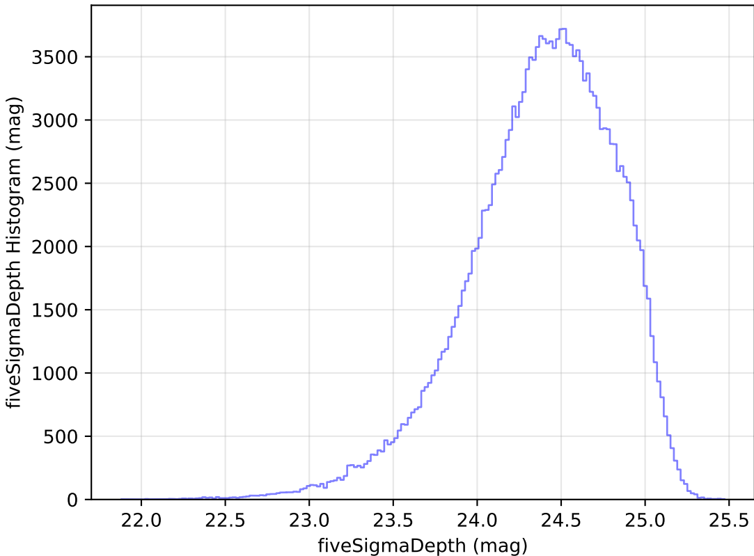
ddf_loaded_fl1_v3.4_10yrs g: fiveSigmaDepth Histogram
