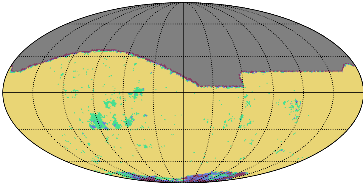
ddf_loaded_fl1_v3.4_10yrs r band: YearCoverage night
