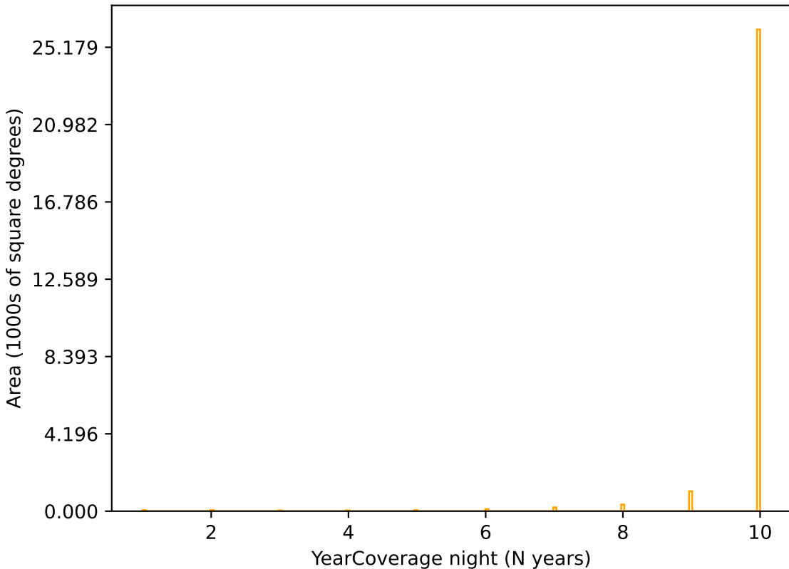
ddf_loaded_fl1_v3.4_10yrs r band: YearCoverage night
