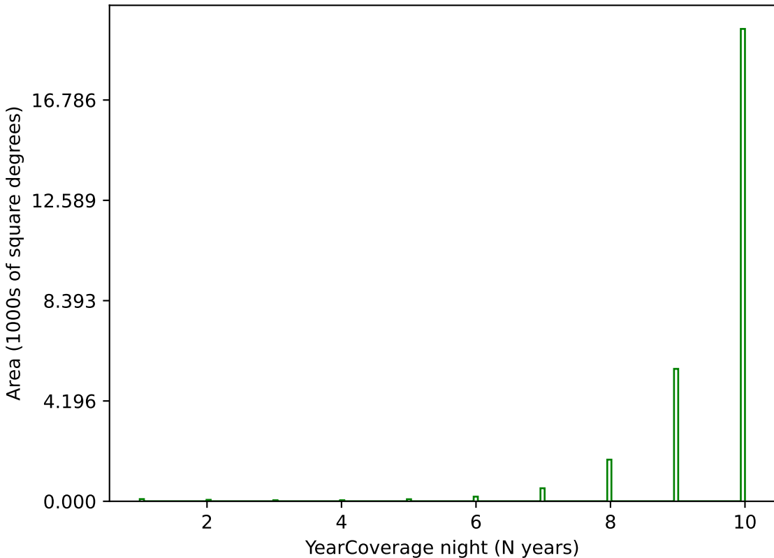
ddf_loaded_fl1_v3.4_10yrs g band: YearCoverage night
