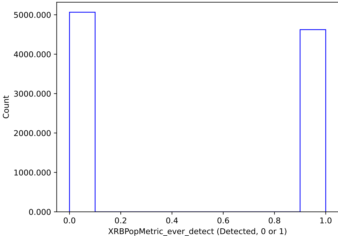
ddf_loaded_fl1_v3.4_10yrs : XRBPoMetric_ever_detect
