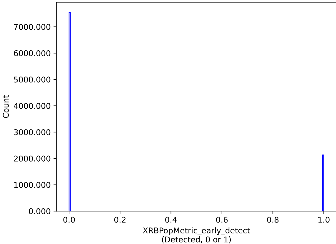
ddf_loaded_fl1_v3.4_10yrs : XRBPoMetric_early_detect
