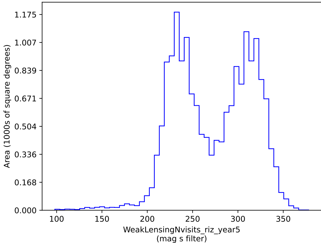
ddf_loaded_fl1_v3.4_10yrs gri band non-DD: WeakLensingNvisits_riz_year5
