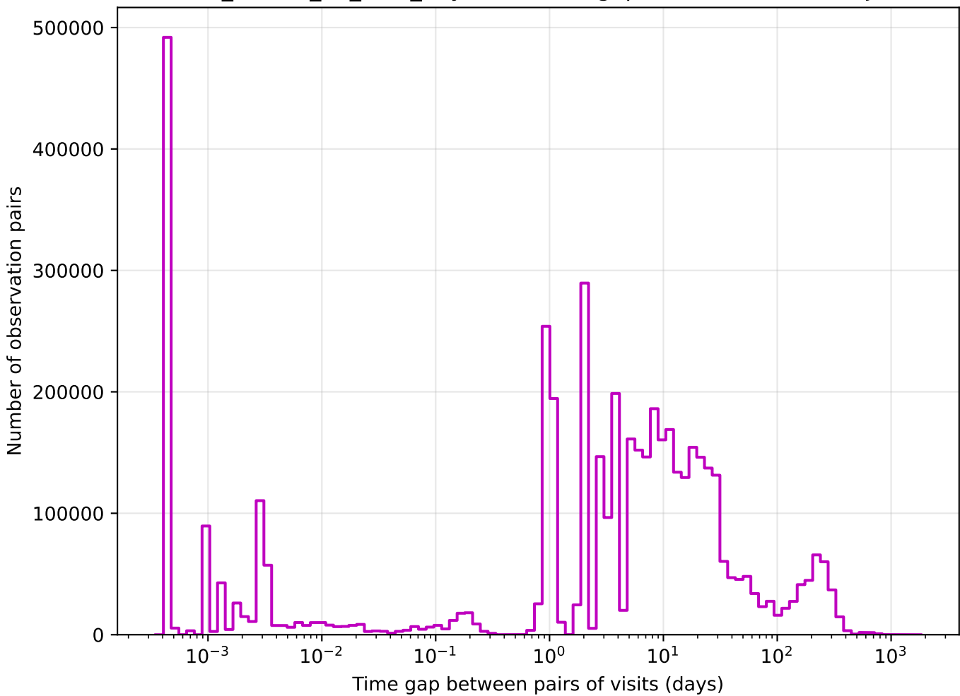
ddf_loaded_fl1_v3.4_10yrs z band: Tgaps observationStartMJD
