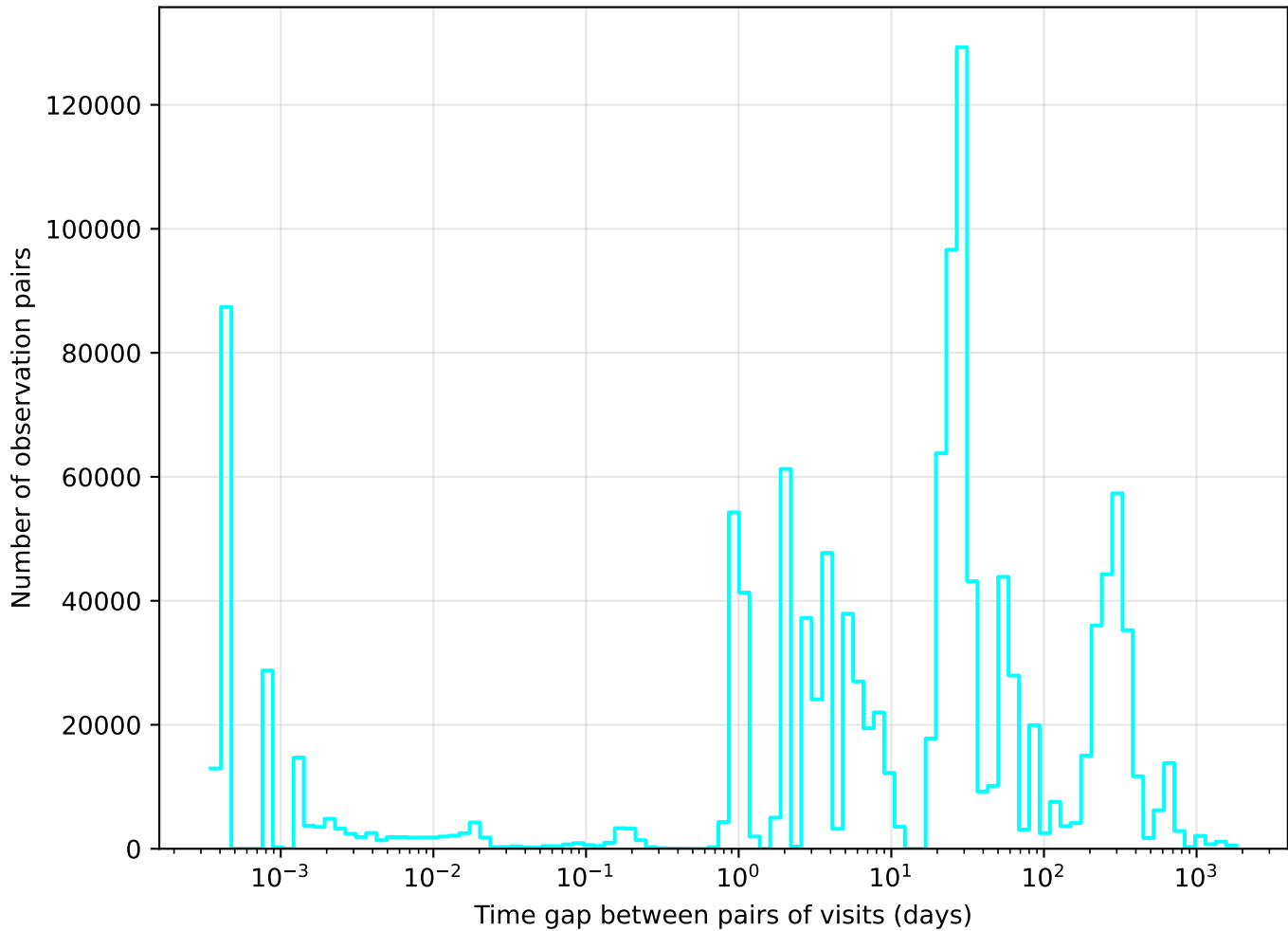
ddf_loaded_fl1_v3.4_10yrs u band: Tgaps observationStartMJD
