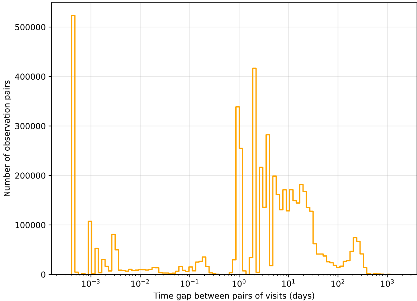
ddf_loaded_fl1_v3.4_10yrs r band: Tgaps observationStartMJD
