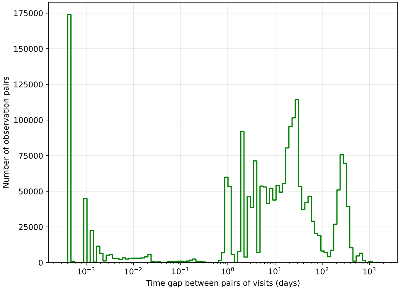
ddf_loaded_fl1_v3.4_10yrs g band: Tgaps observationStartMJD
