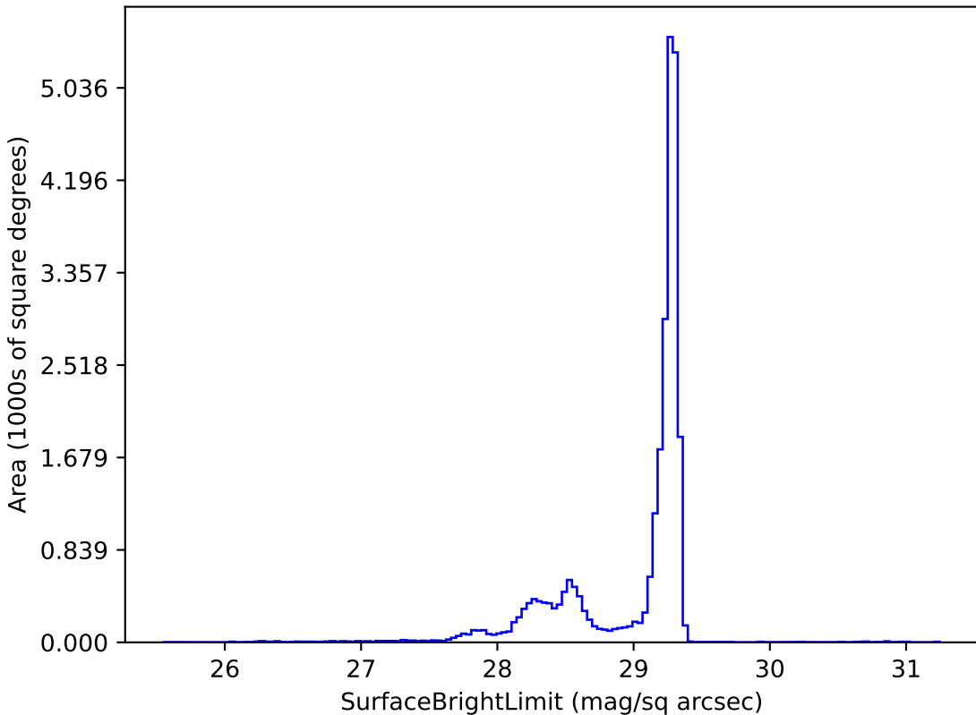
ddf_loaded_fl1_v3.4_10yrs z: SurfaceBrightLimit
